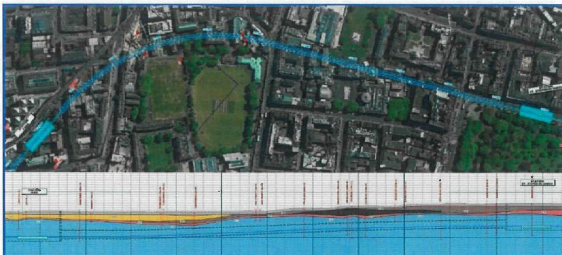
Figure 6. Geological Section (ref. A5.13, Diagram 3.13: Geologic Profile for TBM Drive C8- Tara Station to St. Stephen's Green)
