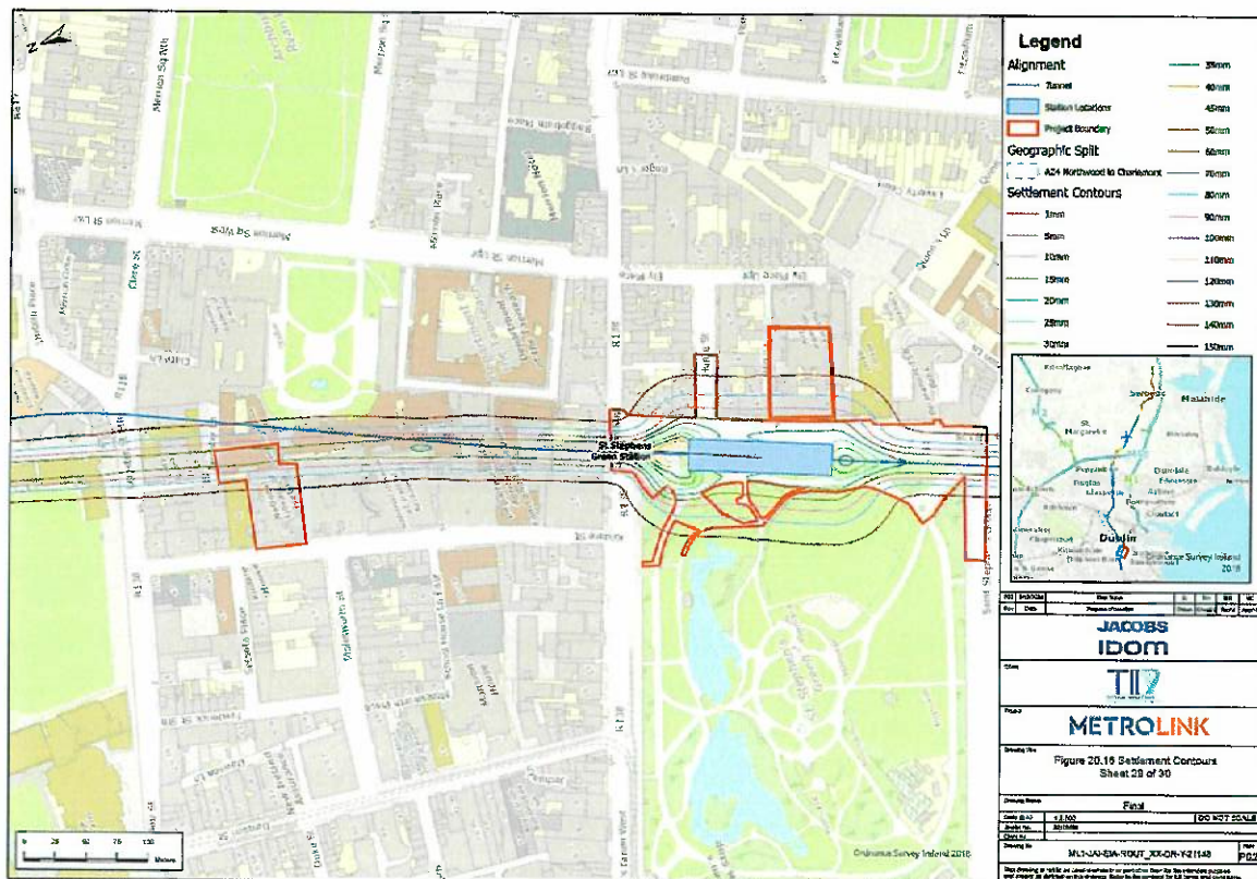
Figure 5. Settlement Contours (Extract from ML1-JAI-EIA-ROUT_XX-DR-Y-21148)
